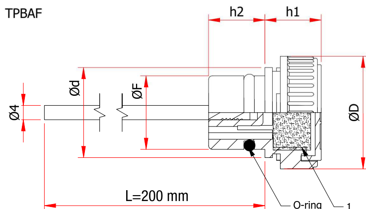
1 = Air filter
